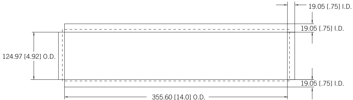
SLEEVE
